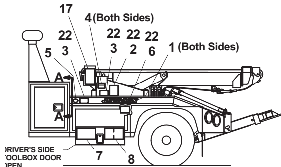
ALUMINUM BODY - DRIVER'S SIDE
